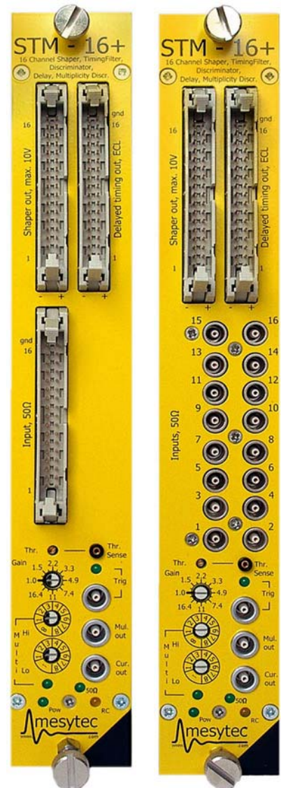
Differential Version Unipolar Version
